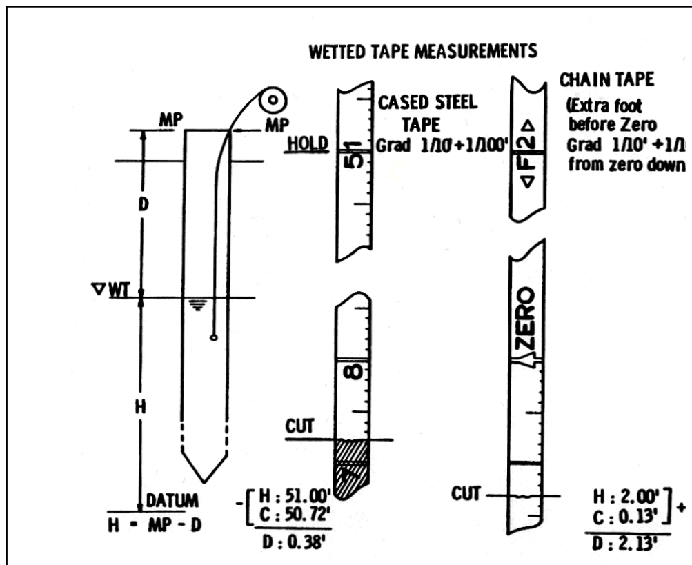
Figure 1. Steel tape.
